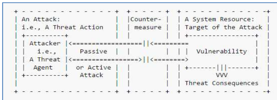
Figure 4: Risk factors of the risk scenario 7
