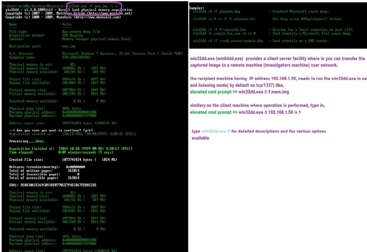
Figure 37: Win32dd tool for Image capturing
